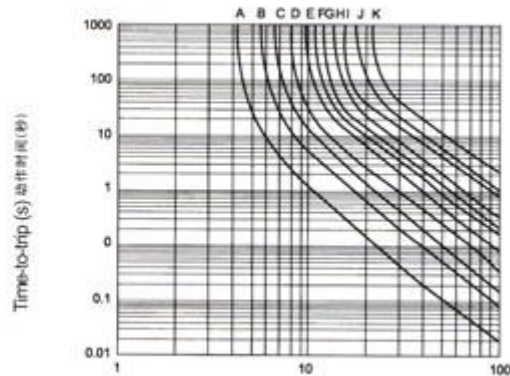
Fault current (A) 故障电流(安培)
